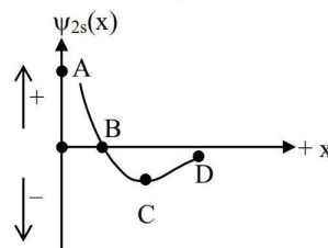
Figure 2. wave function for 2s orbital
